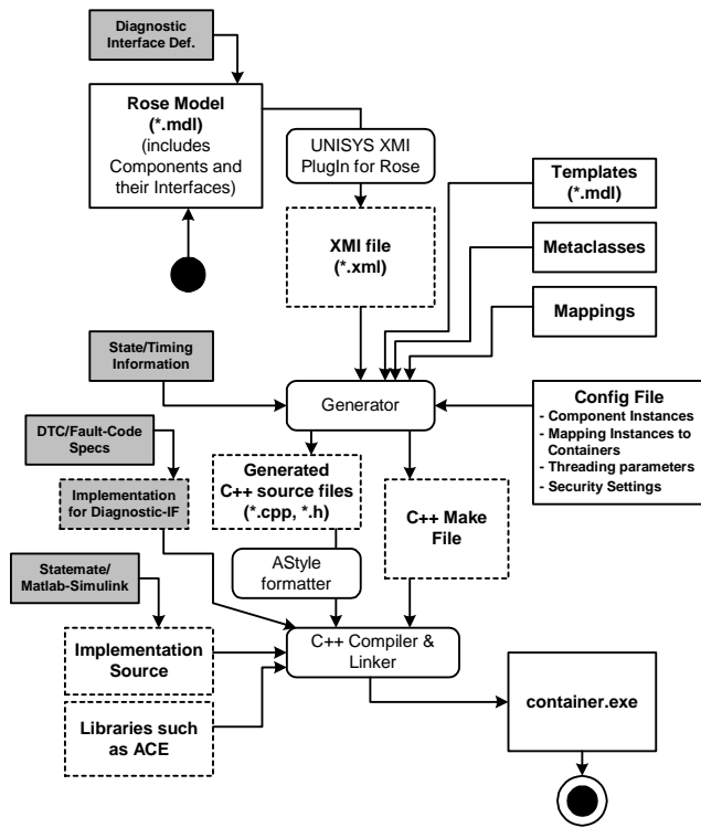
Illustration 5: Diagnostic-specific extensions to the tool
