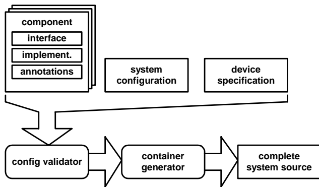
Illustration 2: The proposed solution in a nutshell
