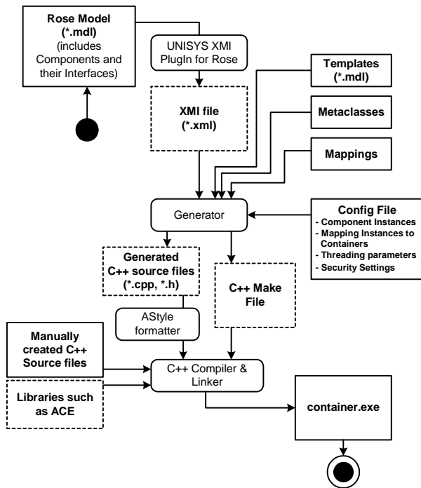
Illustration 3: Prototype implementation structure
